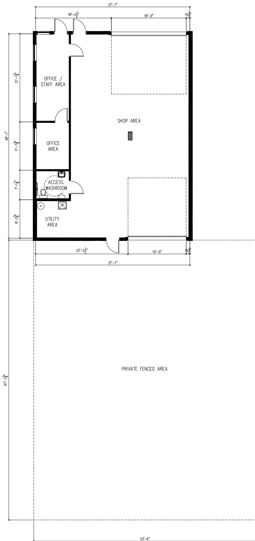
① MAIN FLOOR PLAN TYPE A TYPICAL SINGLE PLAN
